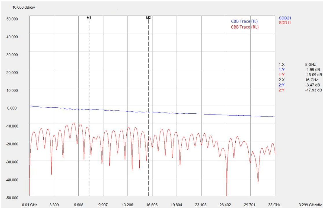
Figure 35. CBB (PCIEG5-M2-TPA3-CBB) characterization without renormalization or gating
