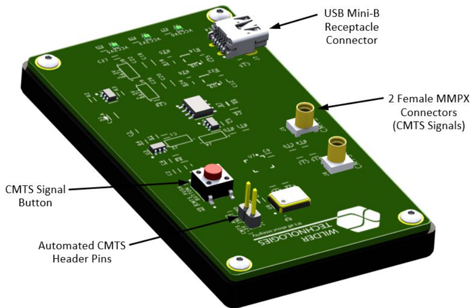
Figure 4. The PCIe Compliance Mode Toggle Signal (CMTS) Fixture
