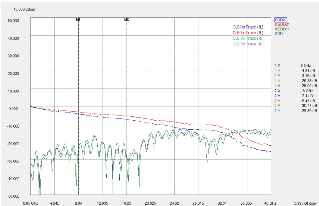
Figure 36. CLB and CBB (PCIEG5-M2-TPA3-CLBCBB) mated insertion and return loss with renormalization and gating
