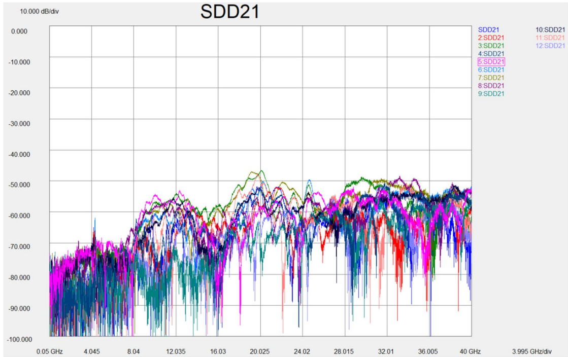
Figure 39. CLB and CBB (PCIEG5-M2-TPA3-CLBCBB) mated FEXT
