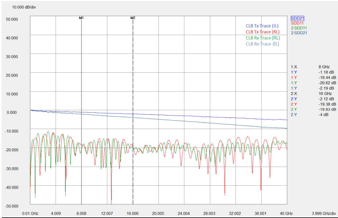
Figure 33. CLB (PCIEG5-M2-TPA3-CLB) characterization without renormalization or gating
