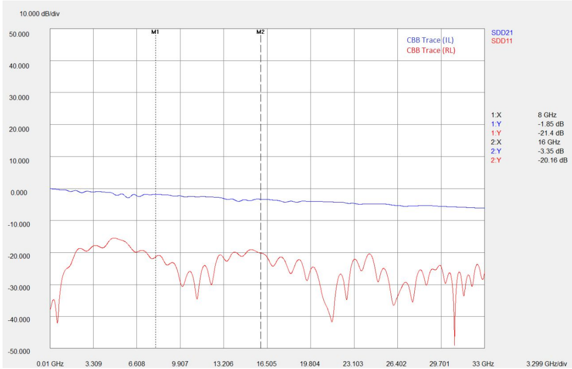
Figure 34. CBB (PCIEG5-M2-TPA3-CBB) characterization with renormalization and gating
